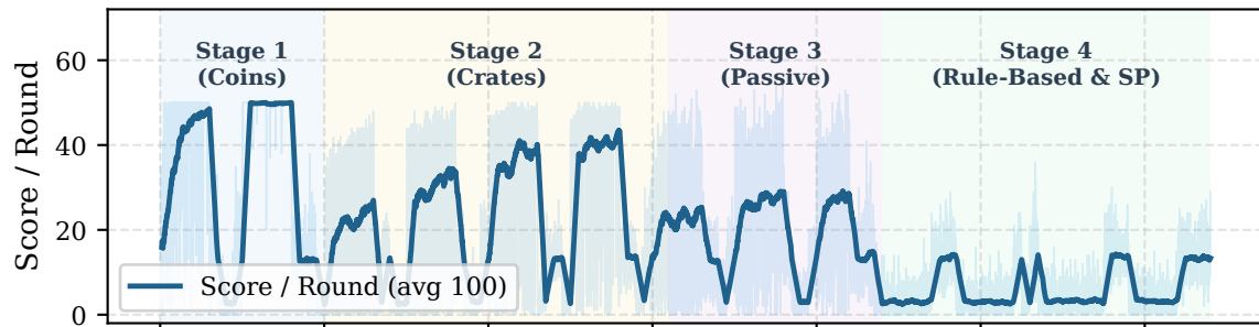
(b) Learning Convergence & Exploration Schedule
