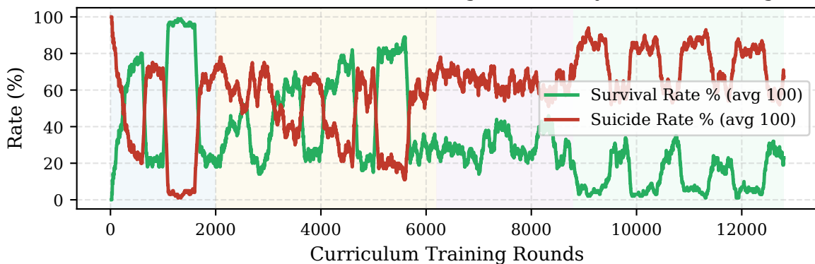
(c) Survival vs. Suicide Rate (Showing Vulnerability without Planning)
